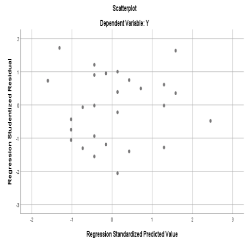
Gambar 3.2 Scatterplot
