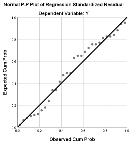
Gambar 3.1 P-P Plot
